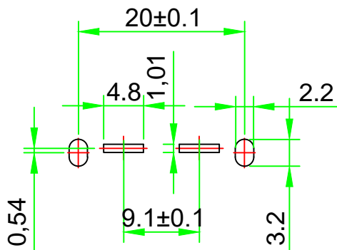
PCB. Mount Hold
