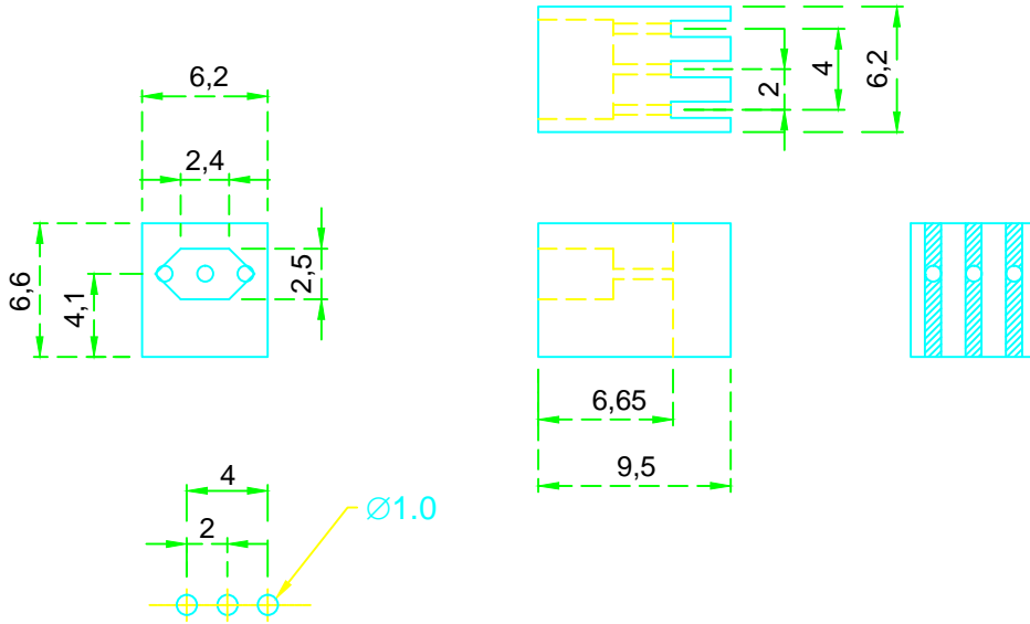
(PCB Layout)
